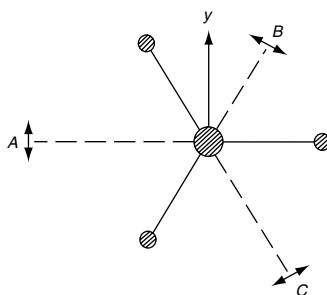
Figure 13-4 ► Three symmetry reflection planes for ammonia.
