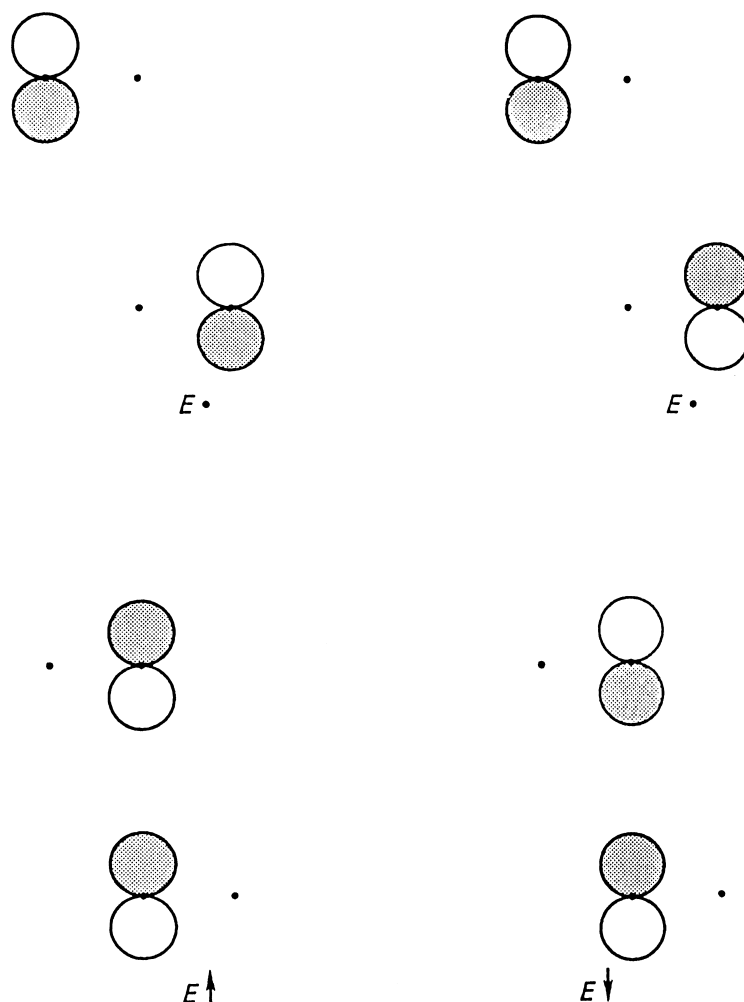
Figure 15-36 ► The four independent unit-cell functions that result from requiring maximum difference in response to the interlayer interaction. E^\bullet indicates no energy change.
