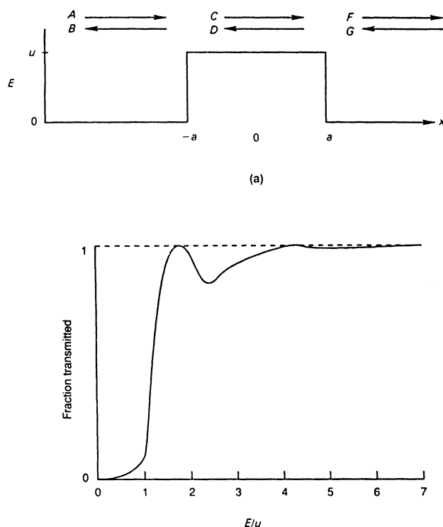
Figure 2-18 ► (a) A rectangular-hill potential of height U and width 2a . (b) Fraction of beam transmitted as a function of E/U , where U = \hbar^2/2\pi^2ma^2 .
