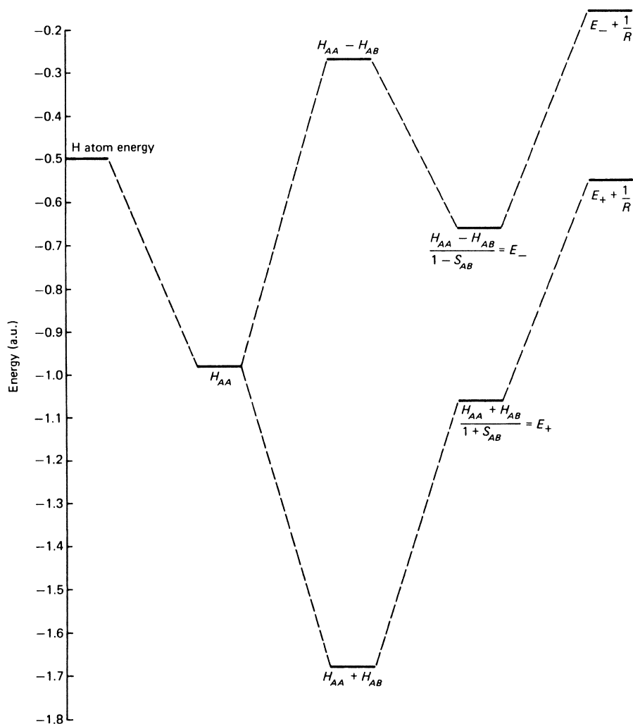
Figure 7-6 ► Contributions to the energy of \text{H}_2^+ at R = 2 a.u. in a minimal basis LCAO-MO calculation.
