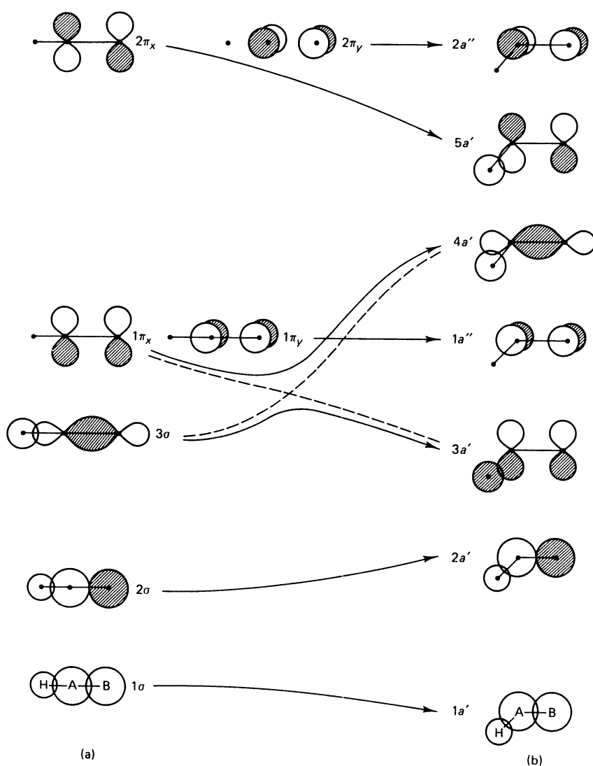
Figure 14-9 ► The Walsh-type diagram for the HAB system: (a) linear C_{\infty v} ; (b) bent C_s . (After Gimarc [6].) Reprinted with permission from Accounts Chem. Res. 7 , 384 (1974). Copyright by the American Chemical Society.
