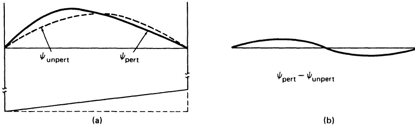
Figure 12-4 ► Sketches of the lowest-energy wavefunction (a) before and after perturbation and (b) the difference between them.
