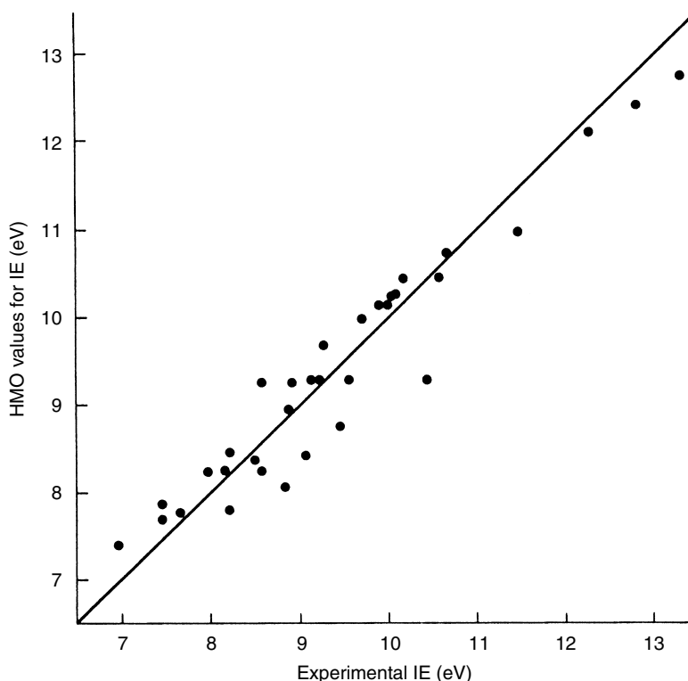
Figure 8-22 ► Experimental ionization energies for alternant and nonalternant hydrocarbons versus HMO orbital energies using \alpha = -6.553 \text{ eV} , \beta = -2.734 \text{ eV} .
