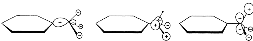
Figure 8-25 ► Three MO symmetry solutions for a methyl group attached to a benzene ring.
