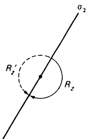
Figure 13-12 ► Effect of a reflection on the direction of \phi .
