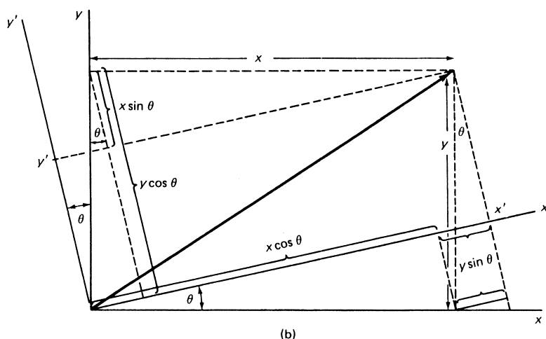
Figure 9-1 ► (a) The vector (3 2). (b) The same vector and its relationship to two Cartesian axis systems.
