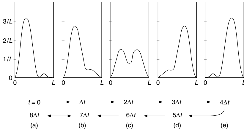
Figure 6-2 ► |\Psi(x, t)|^2 from Eq. (6-38) as it appears at various times.
