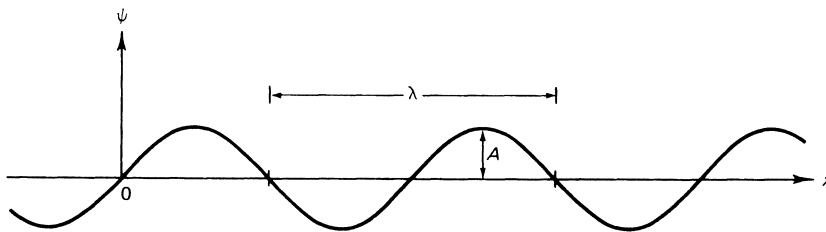
Figure 1-2 ► A harmonic wave at a particular instant in time. A is the amplitude and \lambda is the wavelength.
