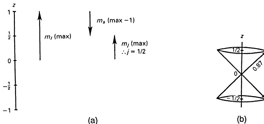
Figure 5-7 ► (a) j = 1/2 , resulting when \mathbf{l} is oriented with its maximum z intercept and \mathbf{s} is oriented in its other orientation (other than as in Fig. 5-6). (b) The two states corresponding to the J = 1/2 vector assuming its possible z intercepts ( 1/2, -1/2 ).
