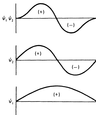
Figure 2-7 ► \psi_1 is symmetric, \psi_2 is antisymmetric, and \psi_1\psi_2 is antisymmetric. The total signed area bounded by the odd functions is zero since complete cancellation of positive and negative components occurs.
