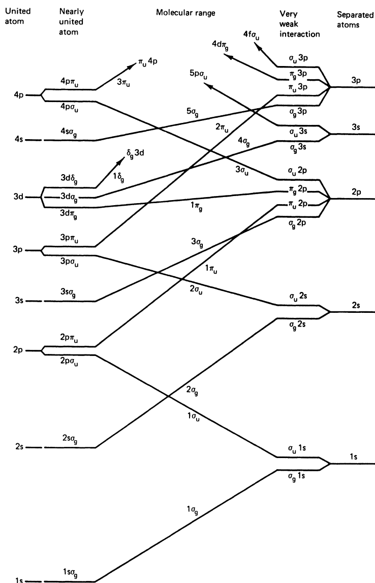
Figure 7-17 ► Correlation diagram between separated-atom orbitals and united-atom orbitals for homonuclear diatomic molecules. Energy ordinate and internuclear separation abscissa are only suggestive. No absolute values are implied by the sketch. [Note: For \text{H}_2^+ \sigma_g 2p correlates with 3d\sigma_g , \sigma_g 3s with 3s\sigma_g . This arises because the separability of the \text{H}_2^+ hamiltonian (in the Born–Oppenheimer approximation) leads to an additional quantum number for this molecule. In essence, the \text{H}_2^+ wavefunction in elliptical coordinates may be written \psi = L(\lambda) M(\mu) e^{im\phi} . The function L may have nodal surfaces of elliptical shape. M may have nodes of hyperbolic shape. In the correlation diagram for \text{H}_2^+ , it is necessary that ellipsoidal nodes correlate with spherical nodes in the united atom, while hyperboloid nodes correlate with hyperboloid nodes (which may be planar). Sketching \sigma_g 2p and \sigma_g 3s and comparing them with 3s\sigma_g and 3d\sigma_g (i.e., 3d_{3z^2-r^2} ) makes clear how this “nodal control” results in what, at first sight, appears to be a violation of the noncrossing rule. For \text{H}_2^+ , modifications for higher-energy states will also be required. For example, 4s\sigma_g will correlate with \sigma_g 4s , not \sigma_g 3p .]
