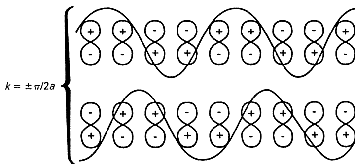
Figure 15-9 ► An alternative to the Bloch sums shown in Fig. 15-8c. These have the same coefficient wavelength but the wave is displaced by a/2 .
