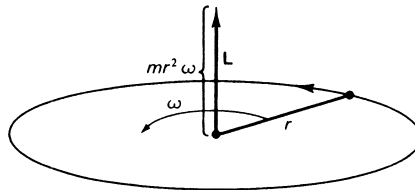
Figure 4-10 ► The angular momentum vector \mathbf{L} for a particle of mass m moving with angular velocity \omega about a circular orbit of radius r in the direction indicated.
