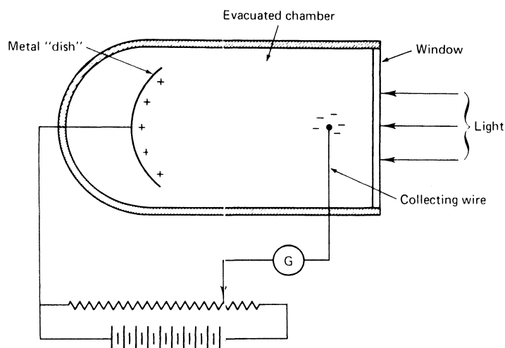
Figure 1-8 ► A phototube.
