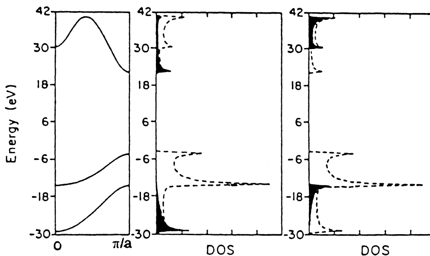
Figure 15-13 ► (a) EHMO band diagram for a linear chain of carbon atoms separated by 140 pm. (b) DOS plot, with 2s AO contributions shaded. (c) DOS plot with 2p_\sigma AO contributions shaded. (From Hoffmann et al. [1].)
