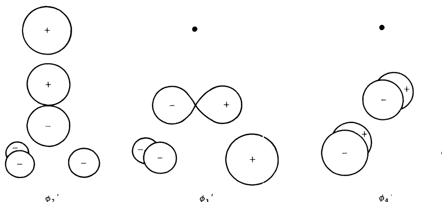
Figure 10-3 ► The three lowest-energy degenerate MOs of methane.
