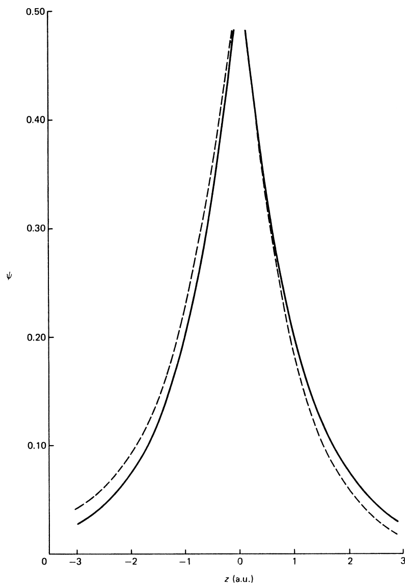
Figure 7-2 ► Values of \psi versus z for 1s state of H atom (—) and for approximate wavefunction given by 0.982 \text{ } 1s - 0.188 \text{ } 2p_z (- - -). The nucleus is at z=0 for each case.
