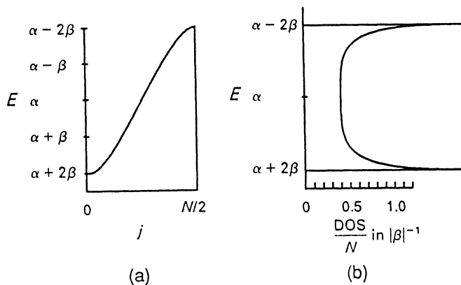
Figure 15-5 ► (a) Hückel energies and (b) density of states for a very large number of carbons in a cycle.
