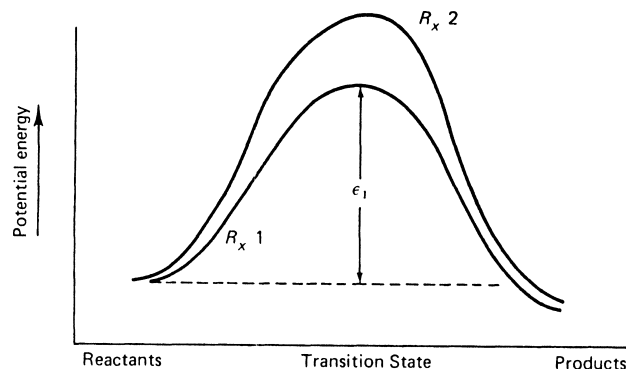
Figure 8-27 ► Generalized energy versus reaction coordinate for reaction at two positions in naphthalene.
