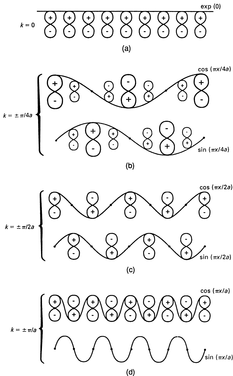
Figure 15-8 ► Coefficient waves times a periodic basis set of one 2p_z AO on each carbon. (a) k = 0 , so the coefficient wave is a constant and the periodic basis is unmodulated. (b)–(d) Plus and minus k -value exponentials are mixed to give trigonometric coefficient waves. In (d), one of these waves has nodes at every carbon so no Bloch sum function exists for this case.
