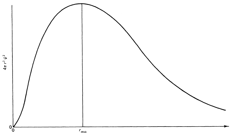
Figure 4-4 ► The volume-weighted probability density for the lowest-energy eigenfunction of the hydrogenlike ion. The most probable value of r occurs at r_{\text{mp}} .
